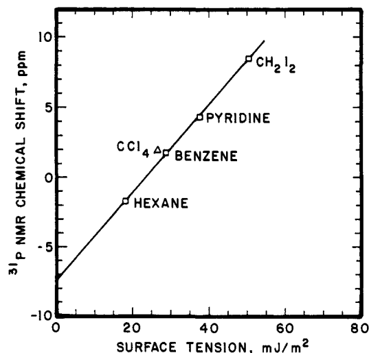
Figure 1. Chemical shifts for the 31 P NMR peak of Et 3 PO due to van der Waals interactions in nonacidic solvents covering a wide range of surface tensions.
