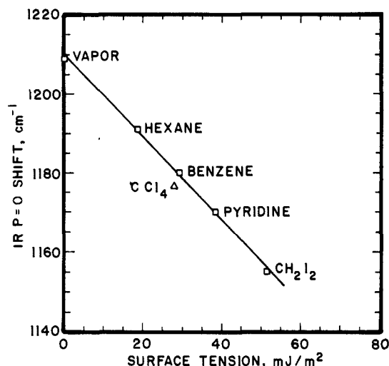
Figure 2. Chemical shifts for the \text{-P=O} infrared stretch frequency of \text{Et}_3\text{PO} in nonacidic solvents covering a wide range of surface tensions.
